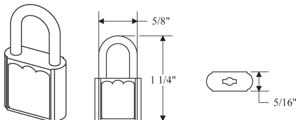
Nickel Plated Pad Lock
